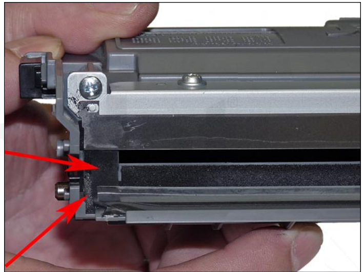
10. Vacuum the doctor blade clean. Until new blades are available, we do not recommend that the doctor blade be removed or the developer roller felt seals disturbed. The doctor blade can be easily cleaned by blowing the excess toner off, and wiping it down with a lint-free cloth. Be very careful not to leave any lint behind!
