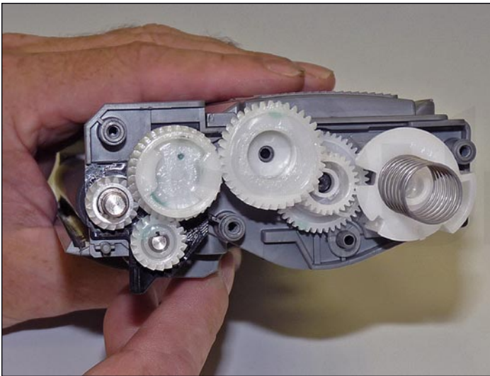
4. Remove the gears and spring as shown.
