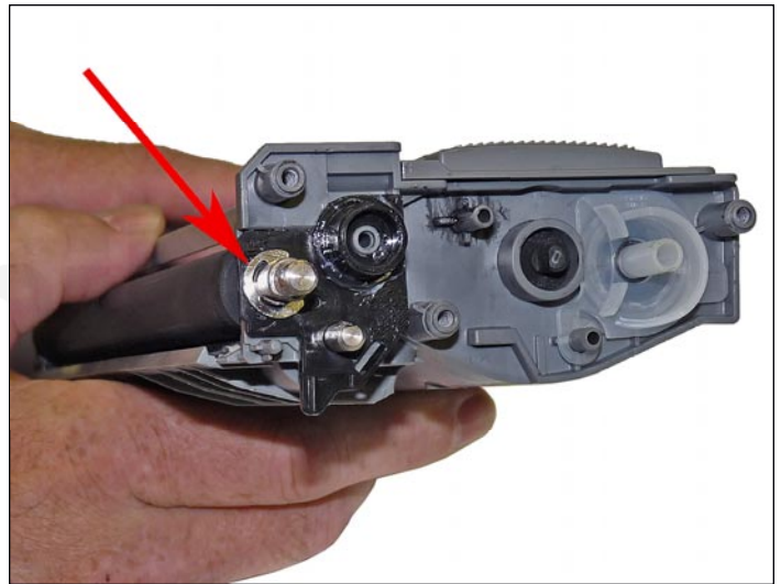
5. Remove the E-ring and the developer roller shaft.
